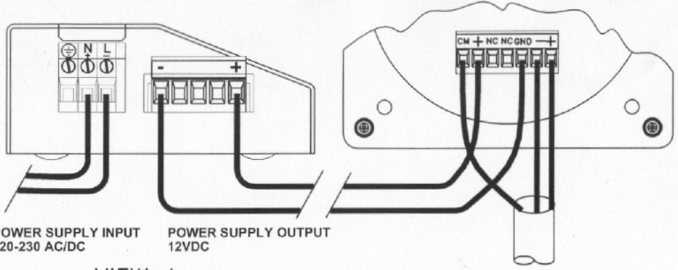
VIEW A
